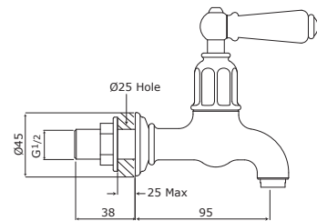
4322 - MAYAN Wall Mounted, with Lever handles 4328 - MAYAN Wall Mounted with Crosshead handles
