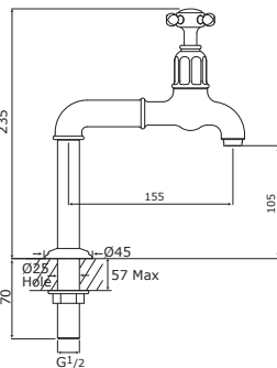
4338 - MAYAN Deck Mounted with Crosshead handles 4332 - MAYAN Deck Mounted with Lever handles
