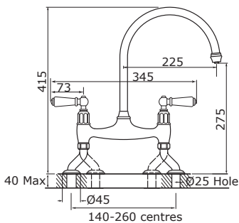
4193 - IONIAN Deck Mounted with Lever handles 4173 - with Rinse 4192 - IONIAN Deck Mounted with Crosshead handles 4172 - with Rinse
