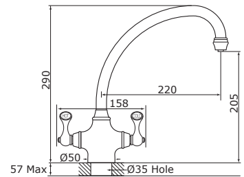
4320 - ETRUSCAN 4350 - with Rinse
