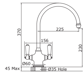
4460 - PHOENICIAN 4360 - with Rinse
